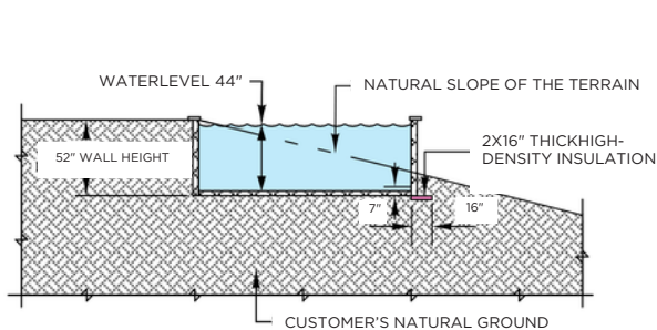
TREVI PRESTIGE EXPOSÉE one to three exposed wall sides more than 24" above the ground
