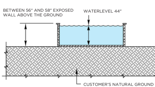
TREVI FUTURA: four exposed wall sides 56" from the ground
