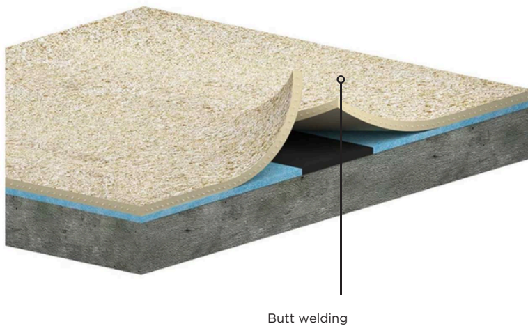
Butt welding
