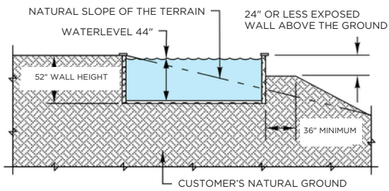
TREVI PRESTIGE EXPOSÉE one to three exposed wall sides at 24" or less from the ground
