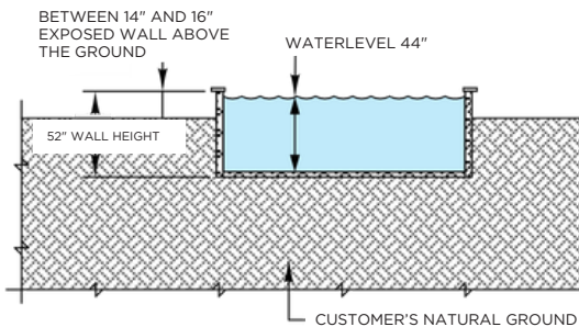
TREVI EUROPEA four exposed wall sides 16" from the ground
