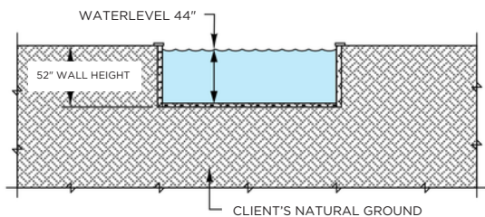
TREVI PRESTIGE installed on a flat terrain
